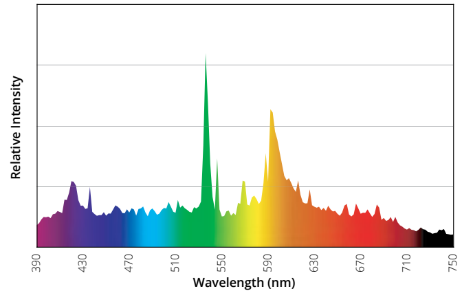
Spectral Power Distribution 4200K
