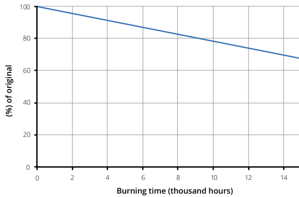
Lumen Maintenance for 150/TD
