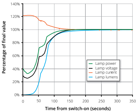
Typical warm-up characteristics for CMH TD 35W
