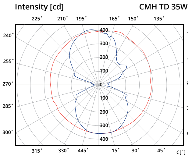
Vertical plane polar intensity curve
