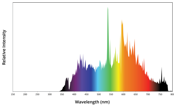
Spectral power distribution CMH MR16 35W 942
