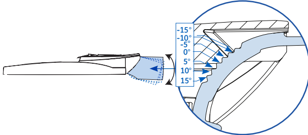
S60 Ø42-60mm pole
