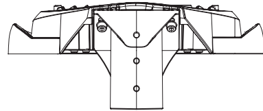
P60 Ø42-60mm pole
